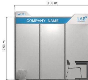
ELEVATION B SCALE 1:50
